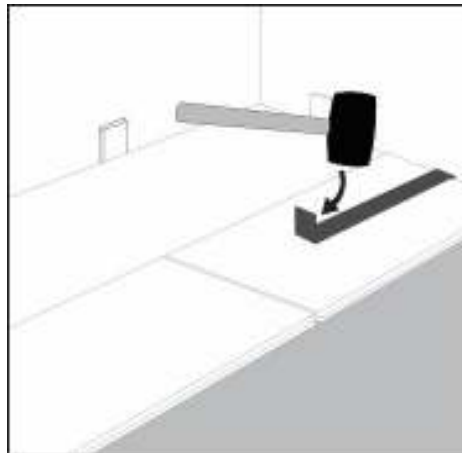
Step 8: Use hammer and pull bar to lock final piece in row. Insert spacer at end of row. Continue installation to final row.
