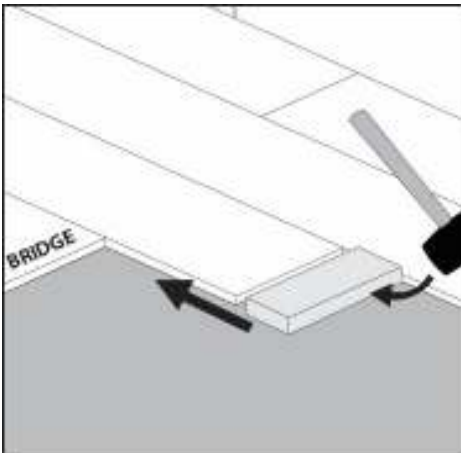
Step 7: Tap end of plank with hammer and tapping block to lock ends of planks together. Remove bridge and continue towards wall until installing the final plank in the row. BE SURE TO TAP ON EDGE OF VINYL SO AS NOT TO DAMAGE LOCKING PROFILE.
